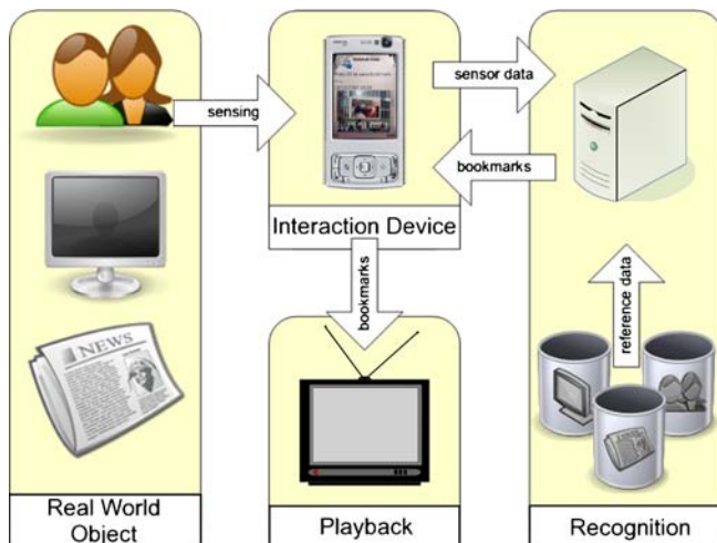
Fig. 1. The central components and their interaction with the contextual bookmark approach
